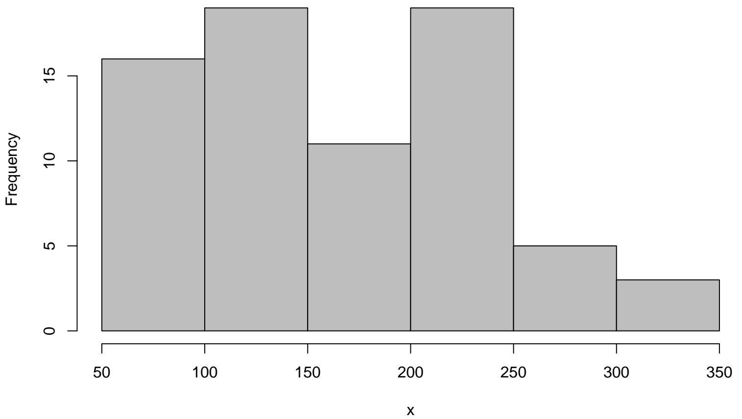
Histogram
