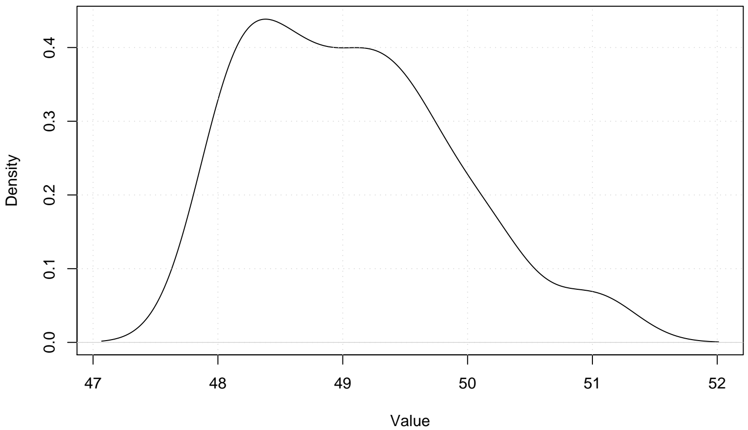
Gaussian Kernel
