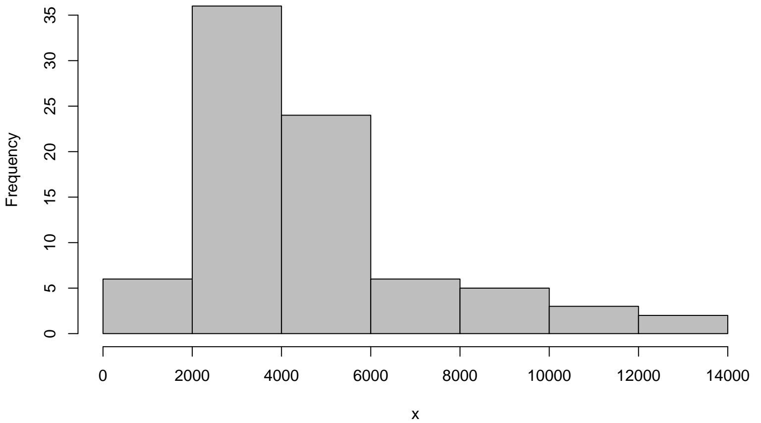
Histogram
