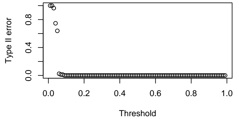
1 - Sensitivity
