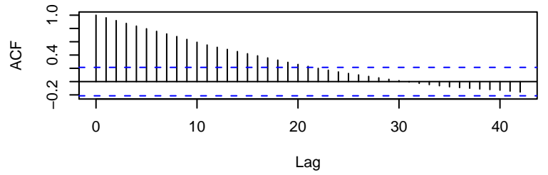
Residuals
