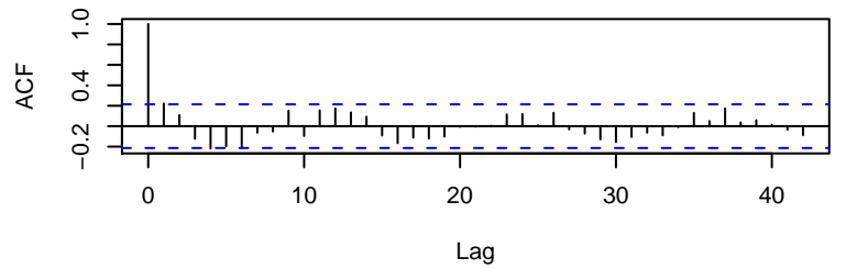
Residuals
