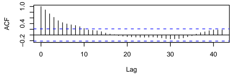
Standardized Residuals
