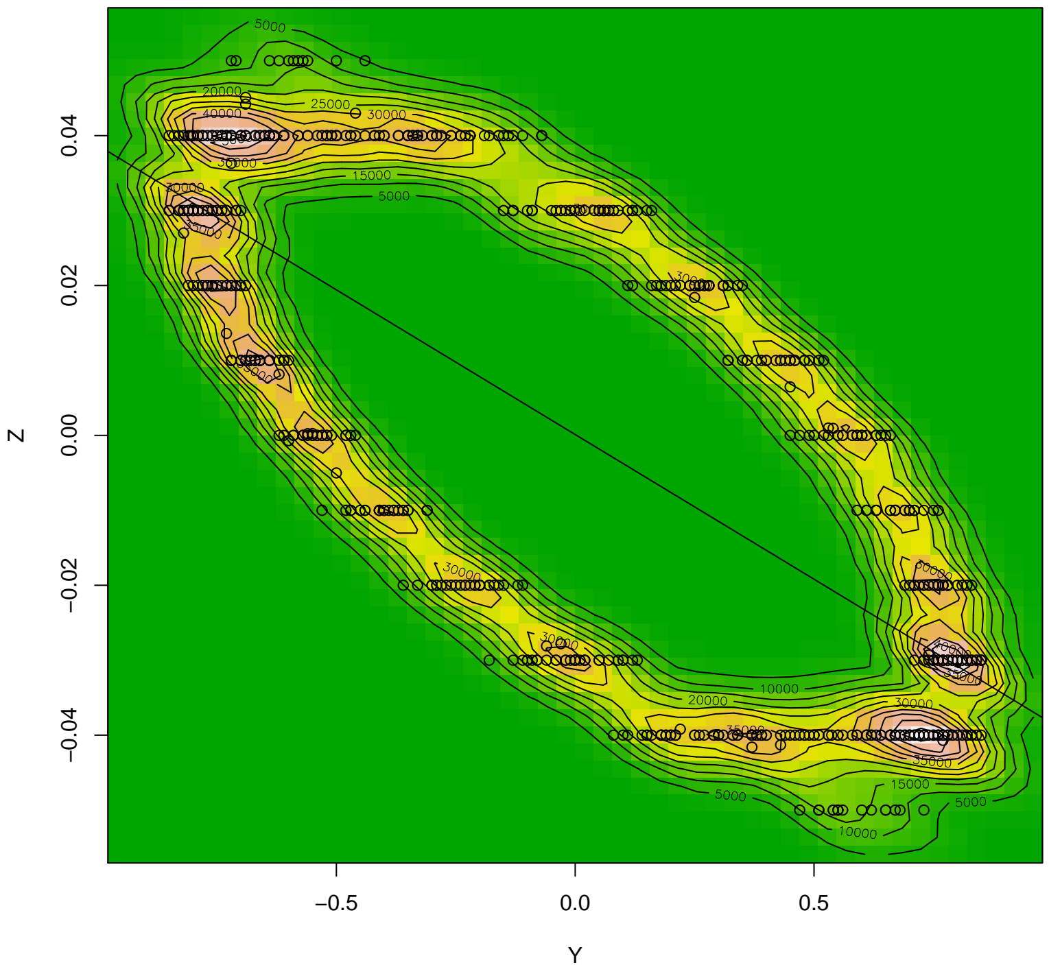
Bivariate Kernel Density Plot (y,z)
