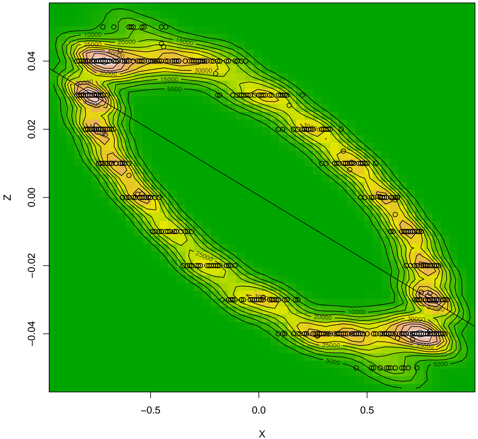
Bivariate Kernel Density Plot (x,z)
