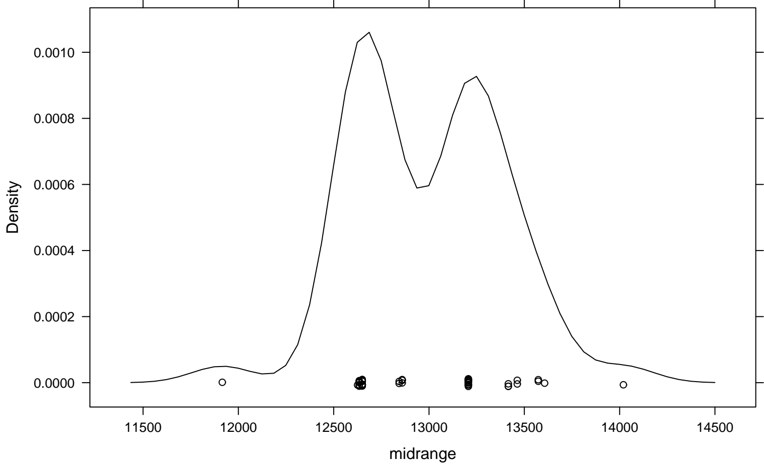
Density Plot
