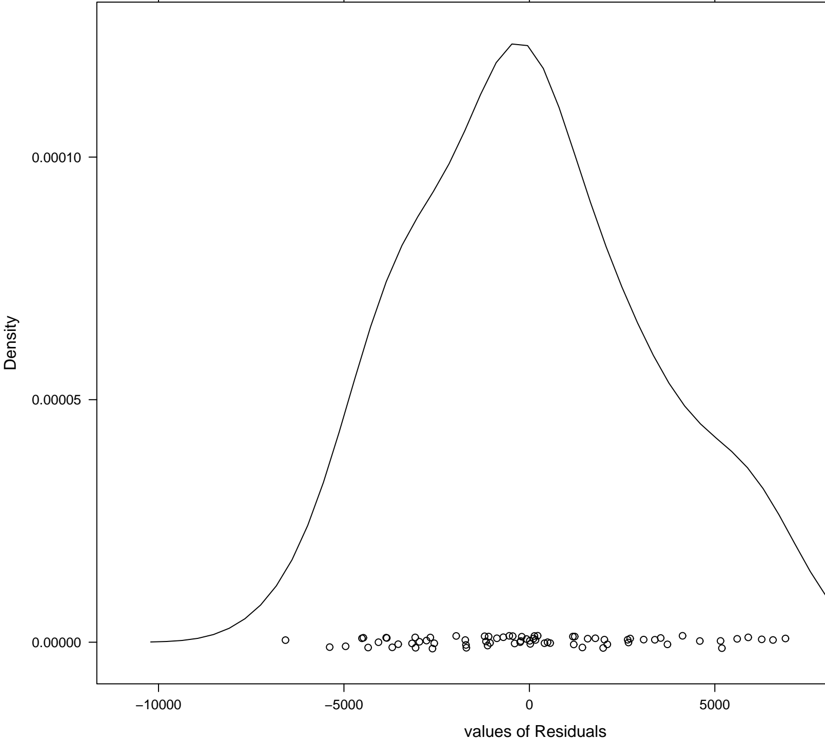
Residual Density Plot
