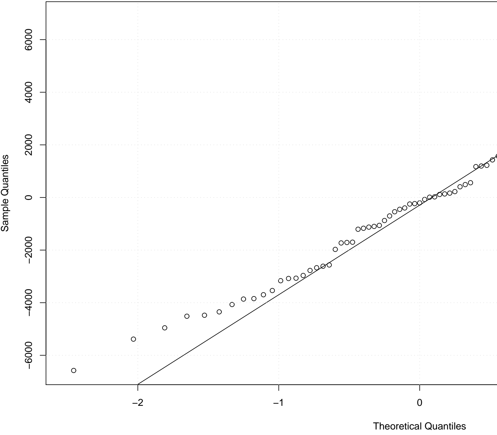
Residual Normal Q-Q Plot
