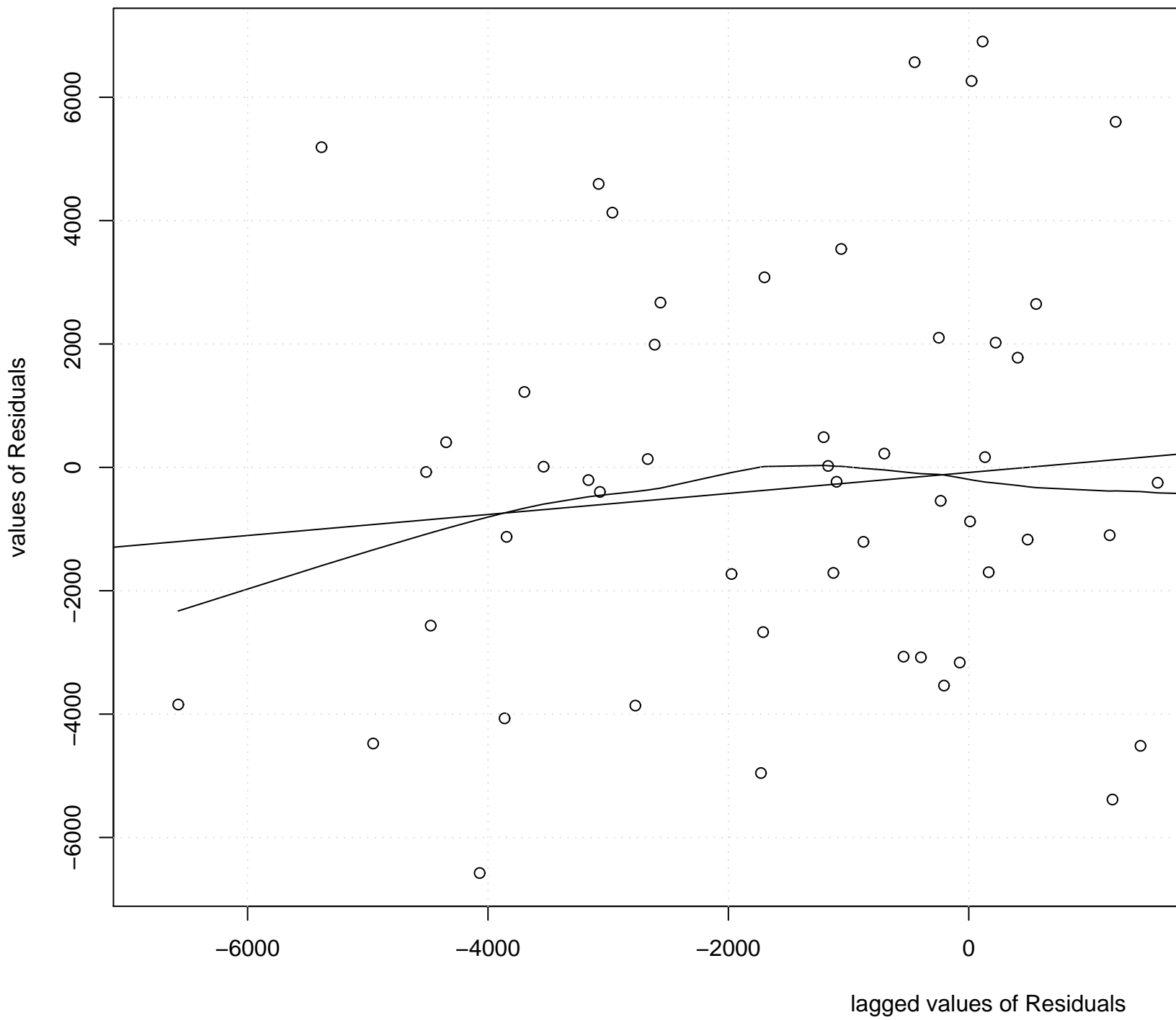
Residual Lag plot, lowess, and regres
