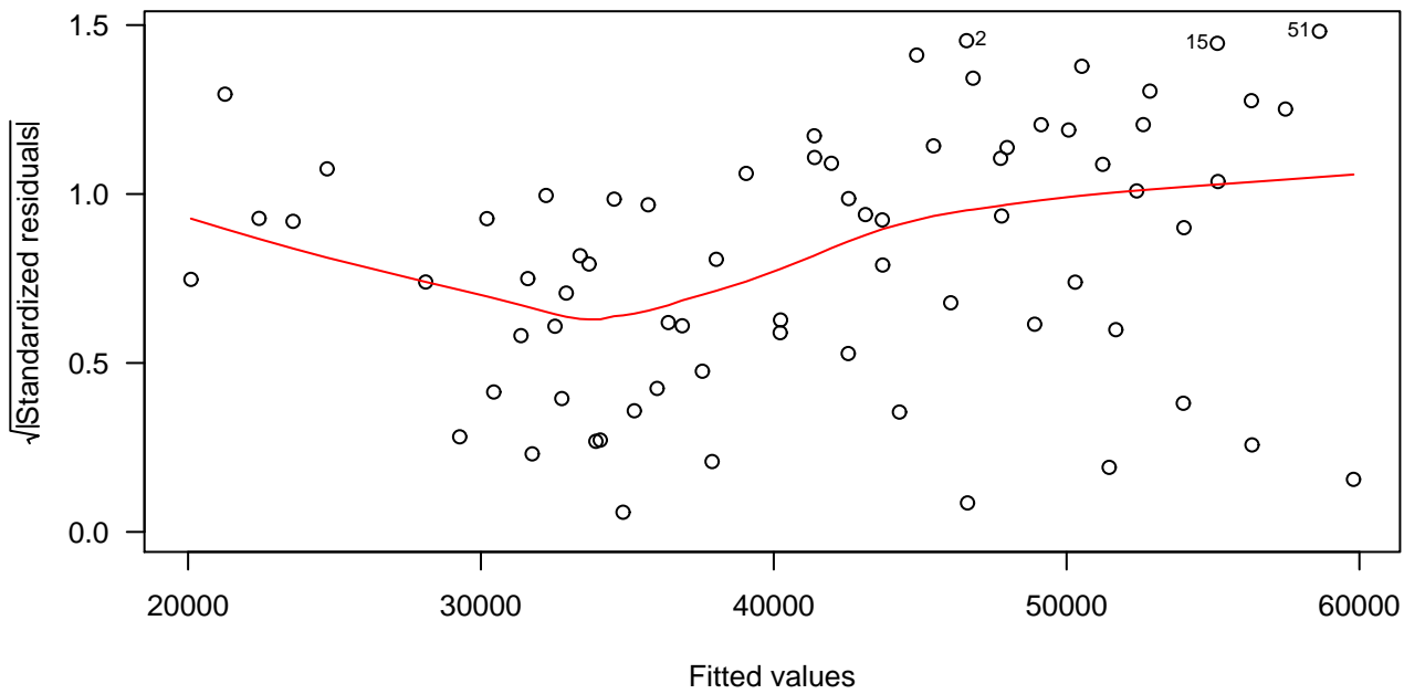
Scale-Location
