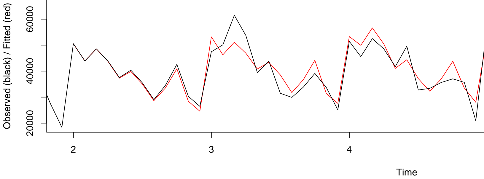
Interpolation Fit of Exponential Smo
