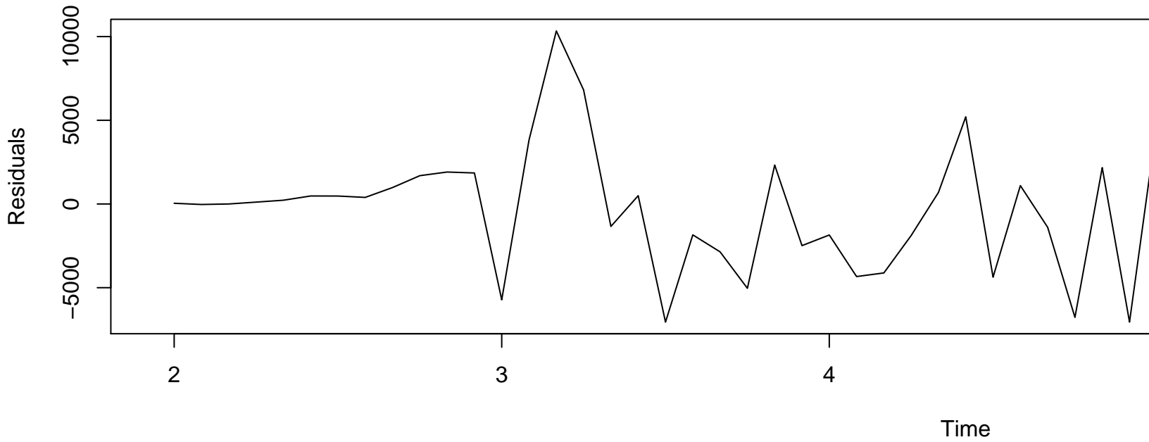
Interpolation Prediction Errors
