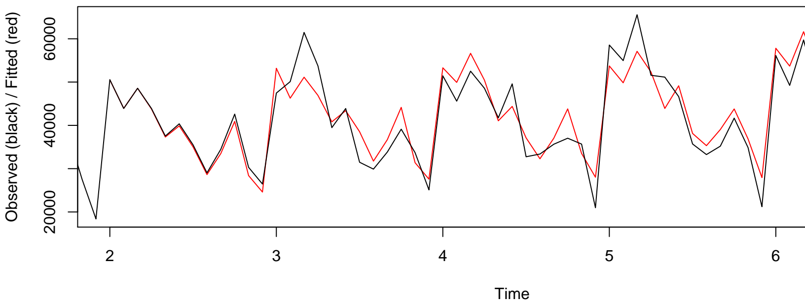
Interpolation Fit of Exponential Smoothing
