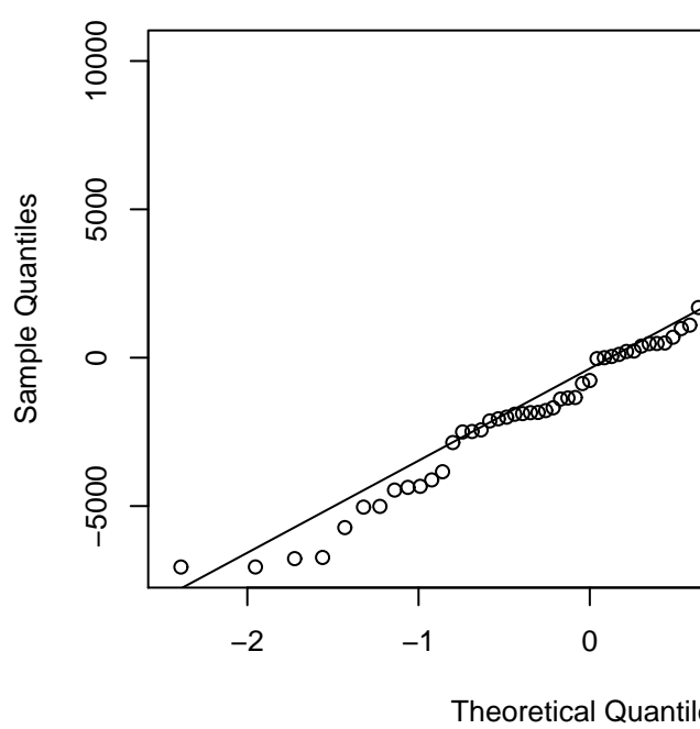
Residual Normal Q-Q
