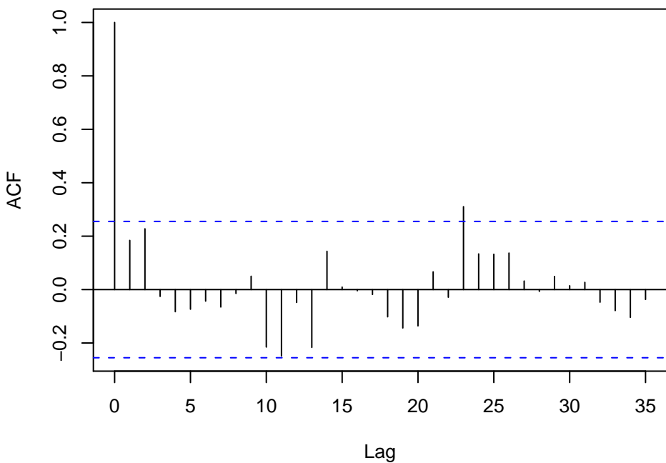
Residual ACF
