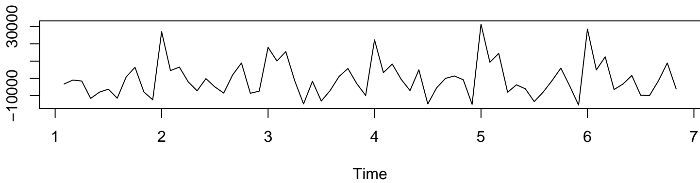
Interpolation Prediction Errors
