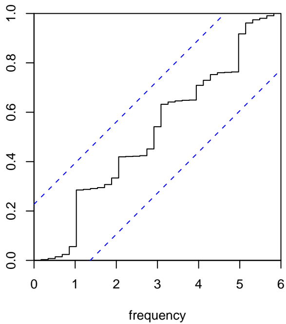
Residual Cumulative Periodogram
