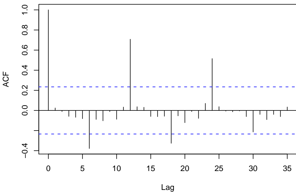
Residual ACF
