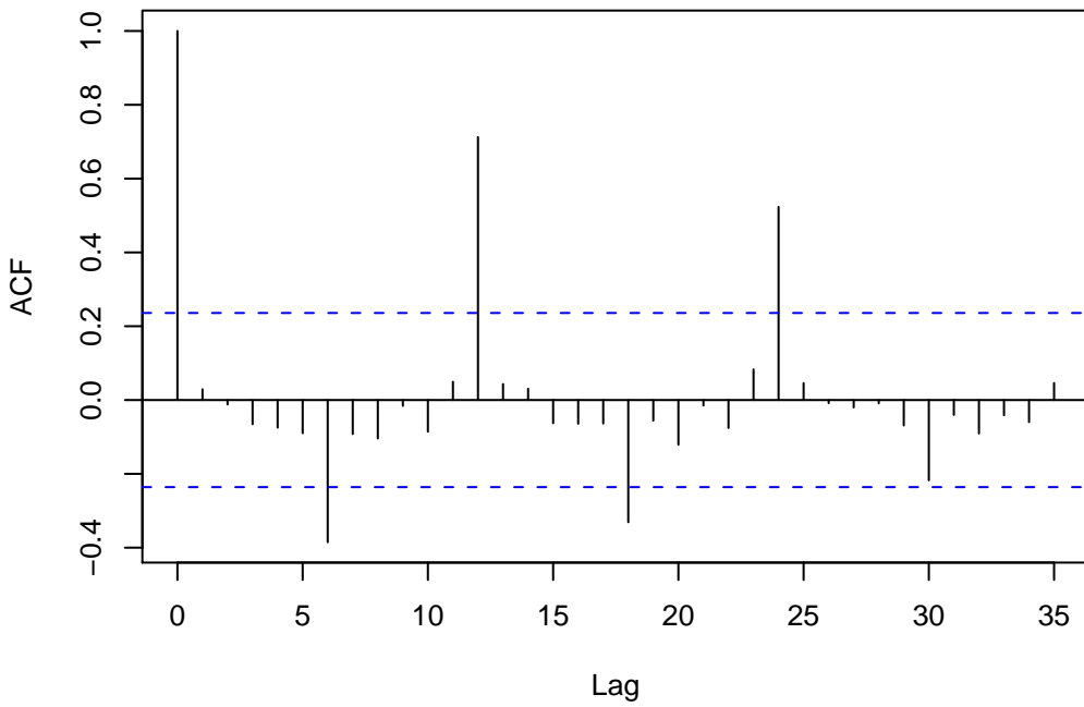
Residual ACF
