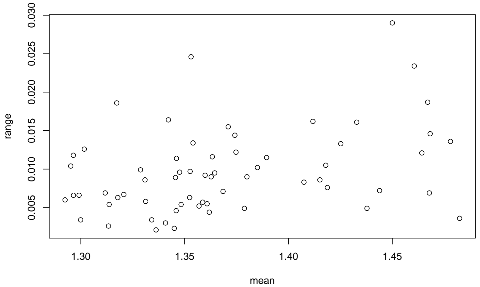
Range-Mean Plot
