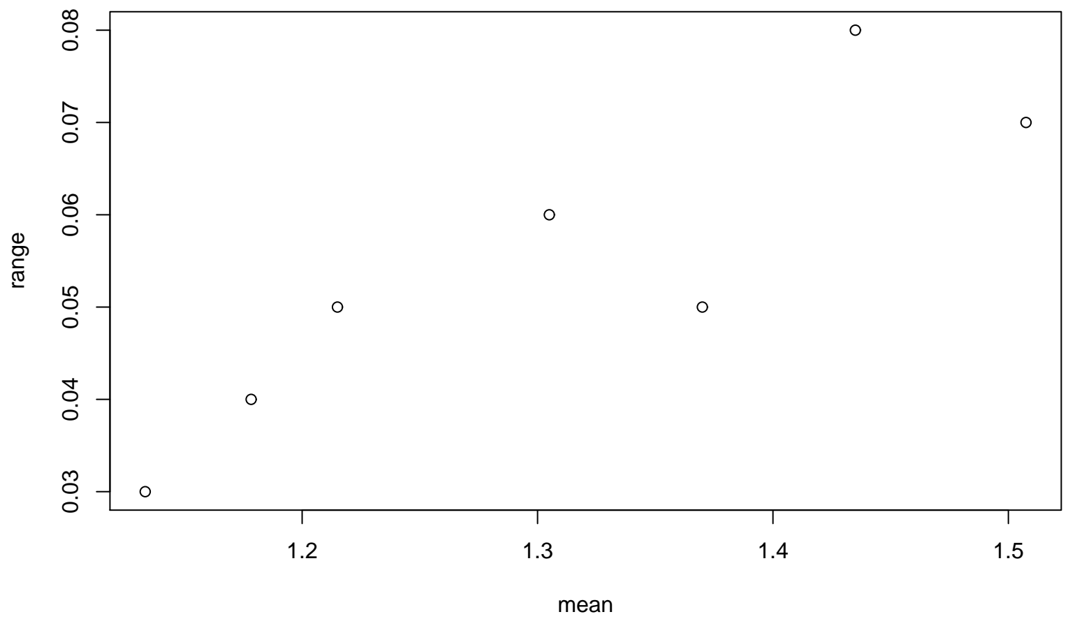
Range-Mean Plot
