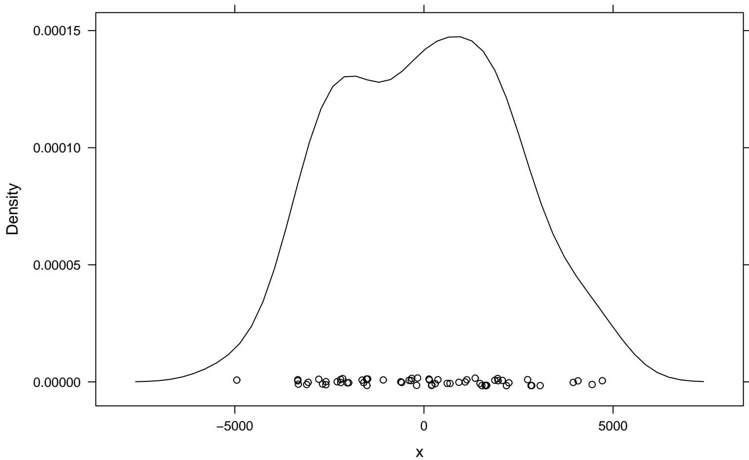
Density Plot
