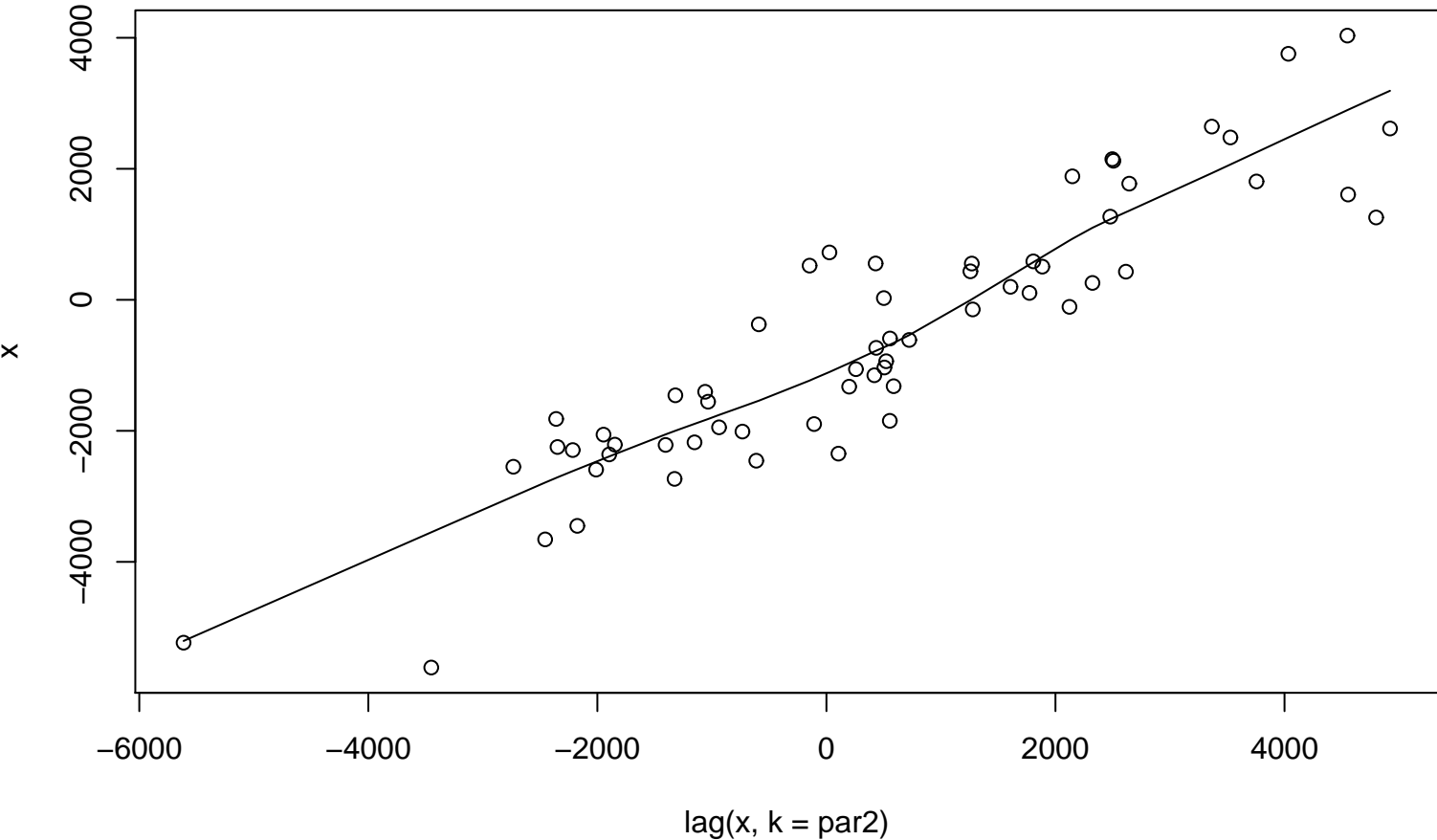
Lag plot (k=12), and lowess
