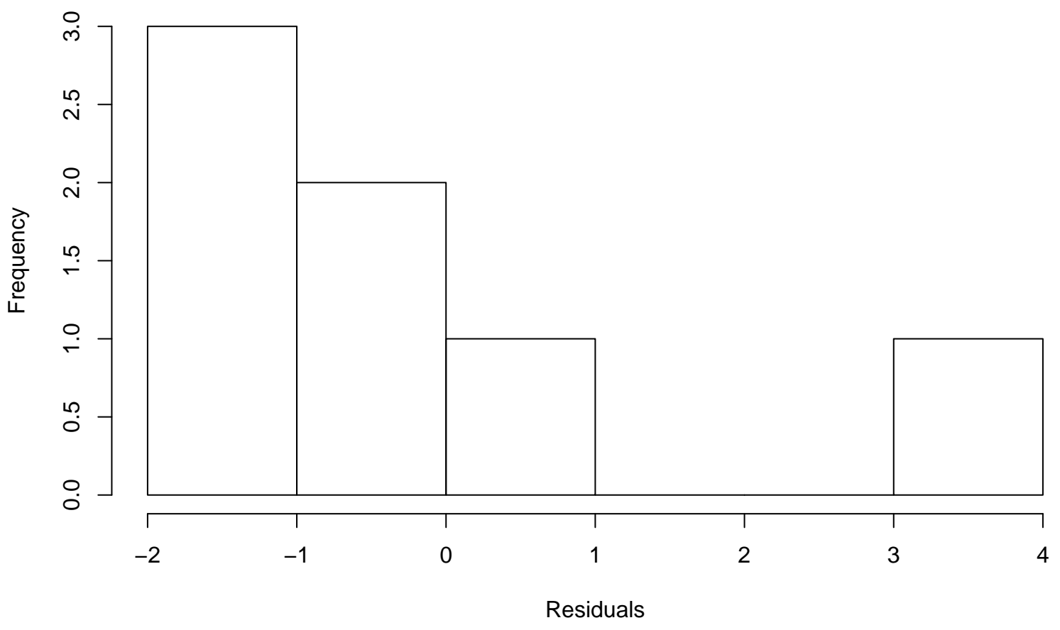
Residual Histogram
