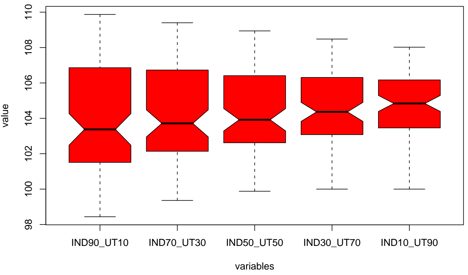
Notched Boxplots
