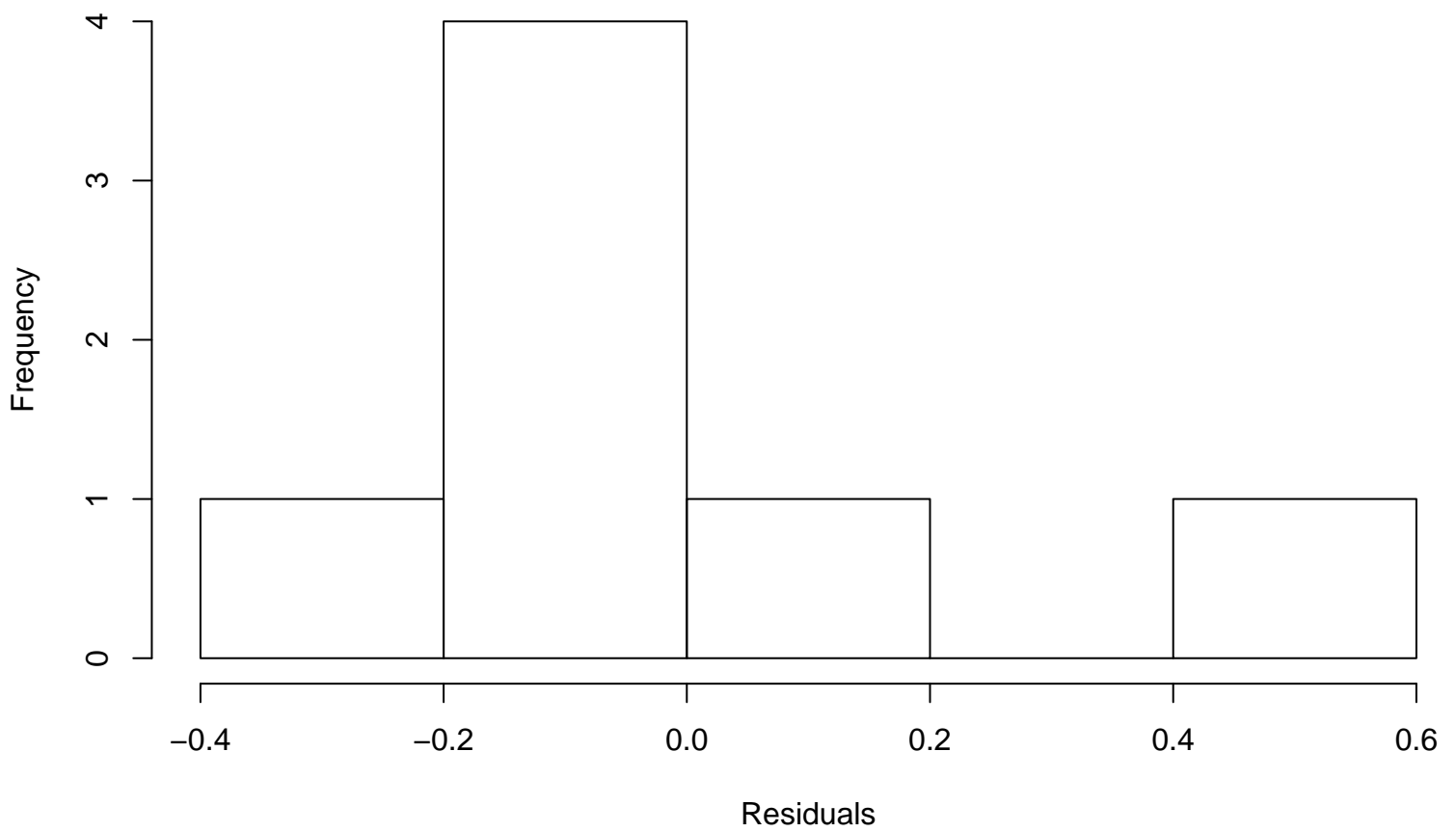
Residual Histogram
