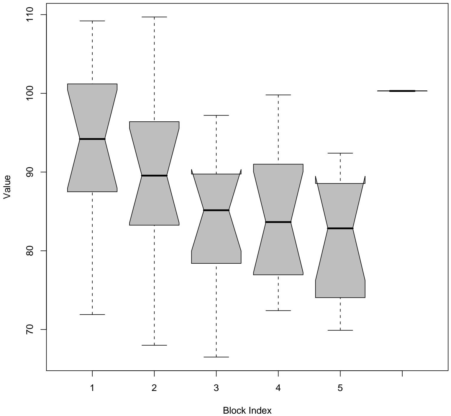
Notched Box Plots – Sequential Blocks
