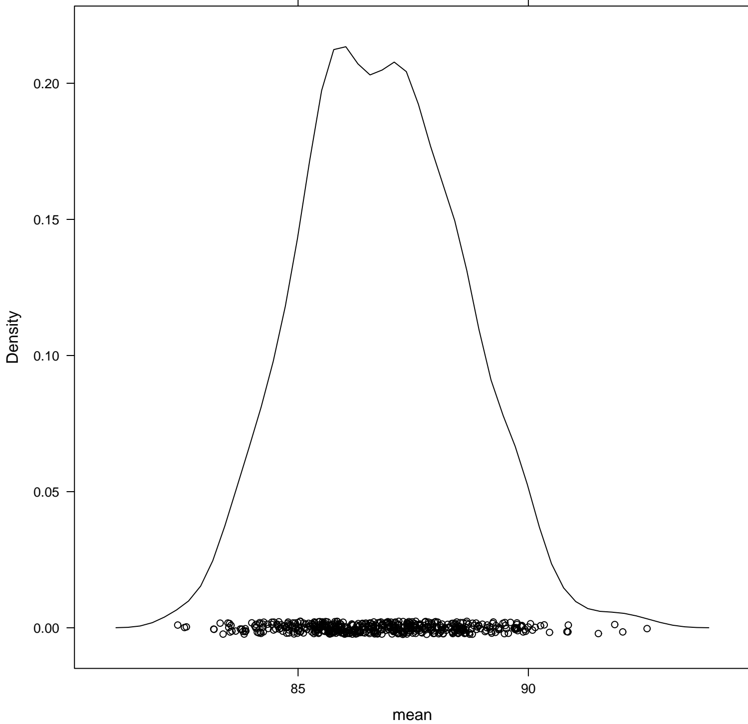
Density Plot
