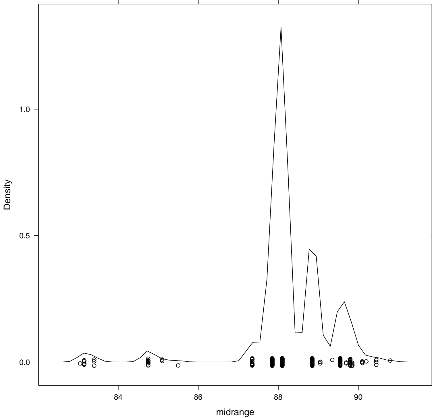
Density Plot
