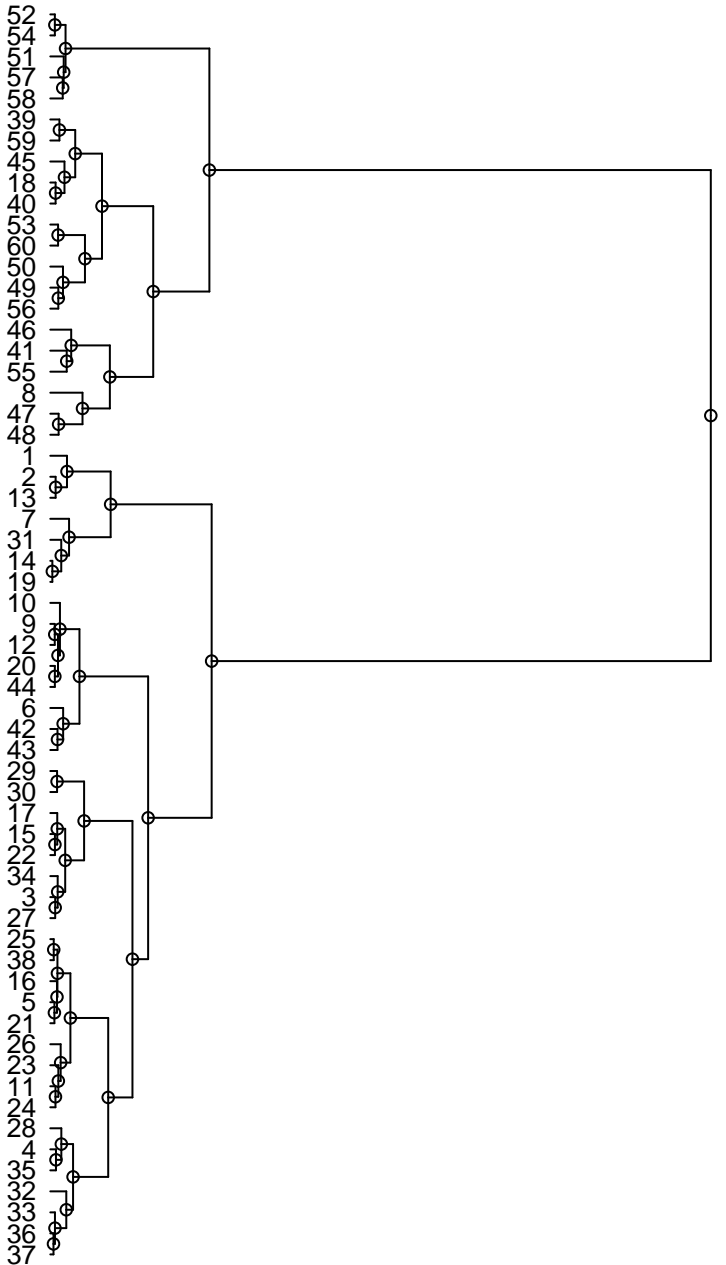
Dendrogram
