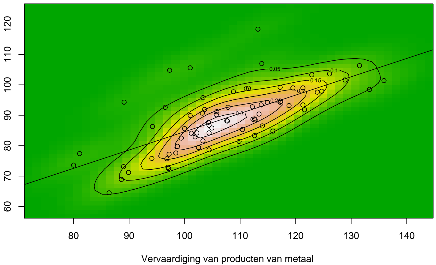
Bivariate Kernel Density Plot (x,y)
