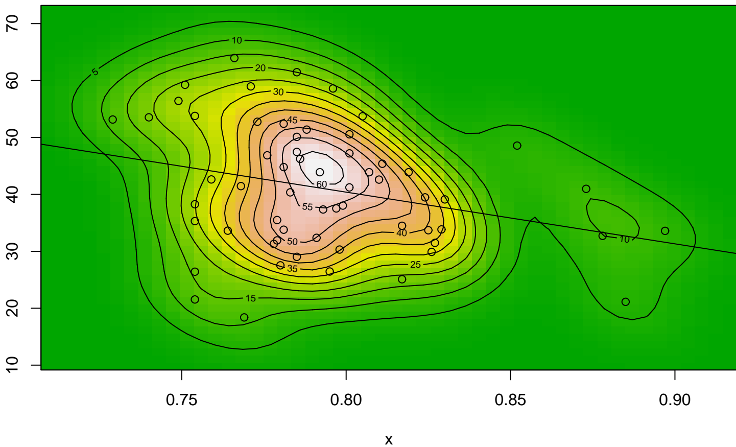
Bivariate Kernel Density
