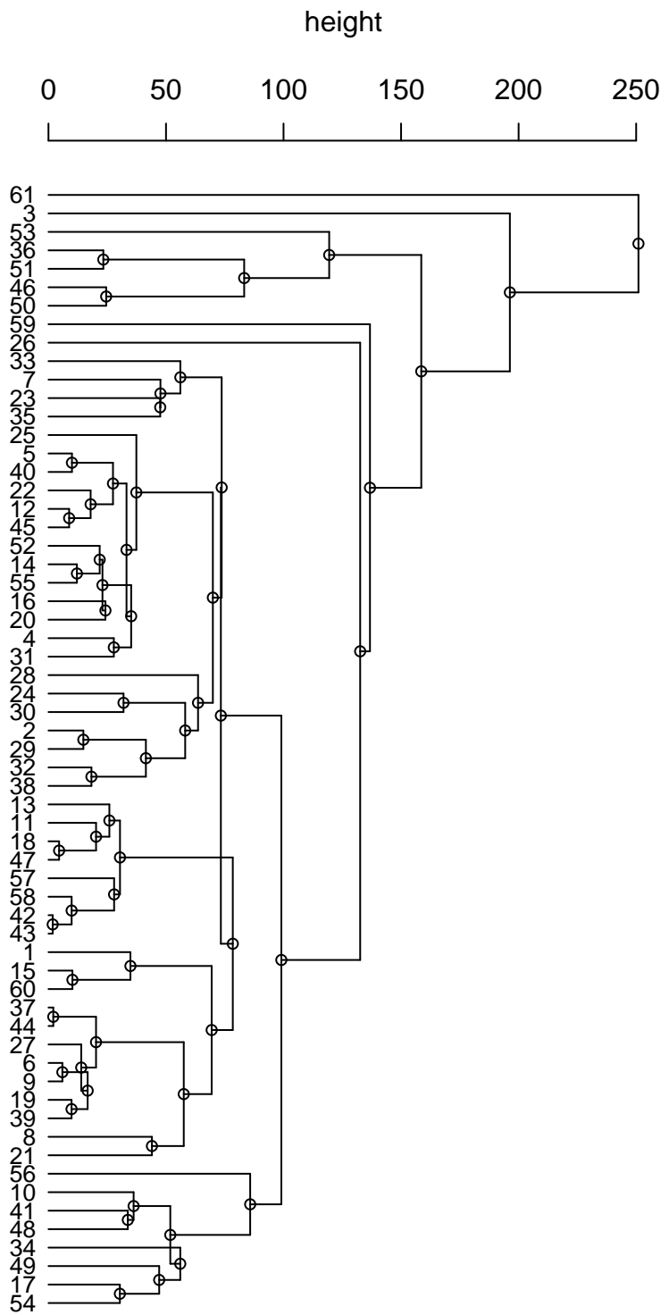
Dendrogram
