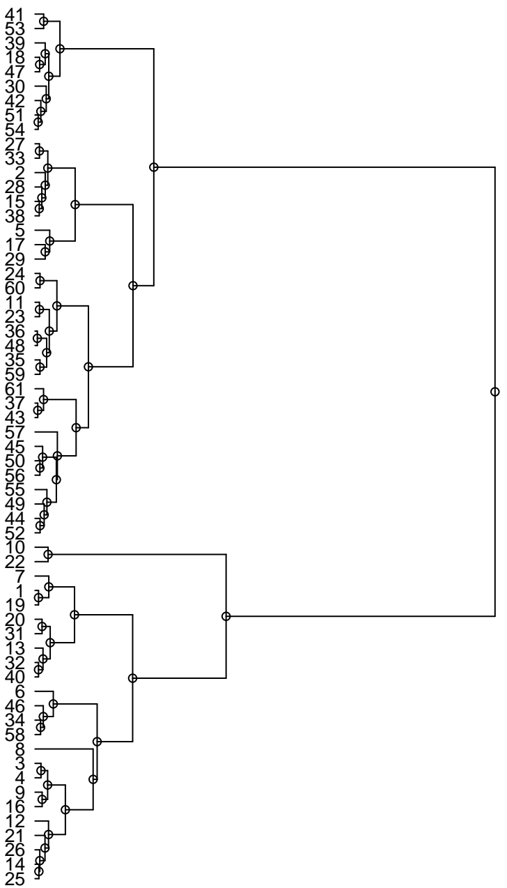
Dendrogram
