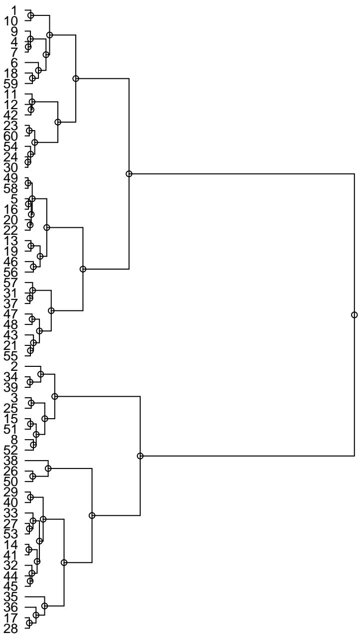
Dendrogram
