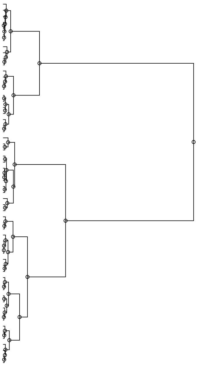
Dendrogram
