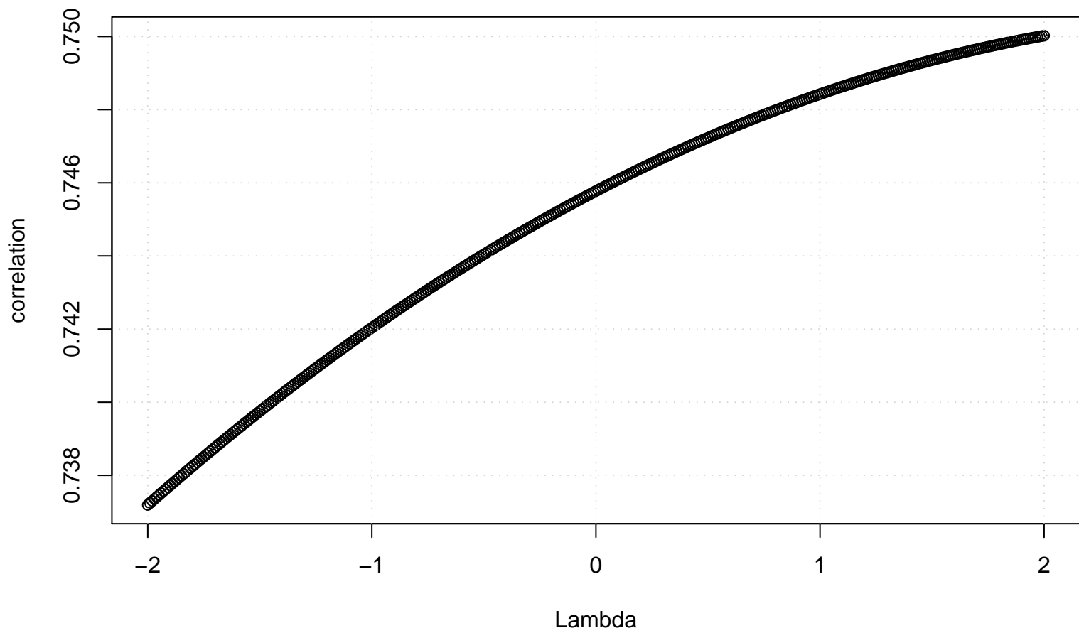
Box-Cox Linearity Plot
