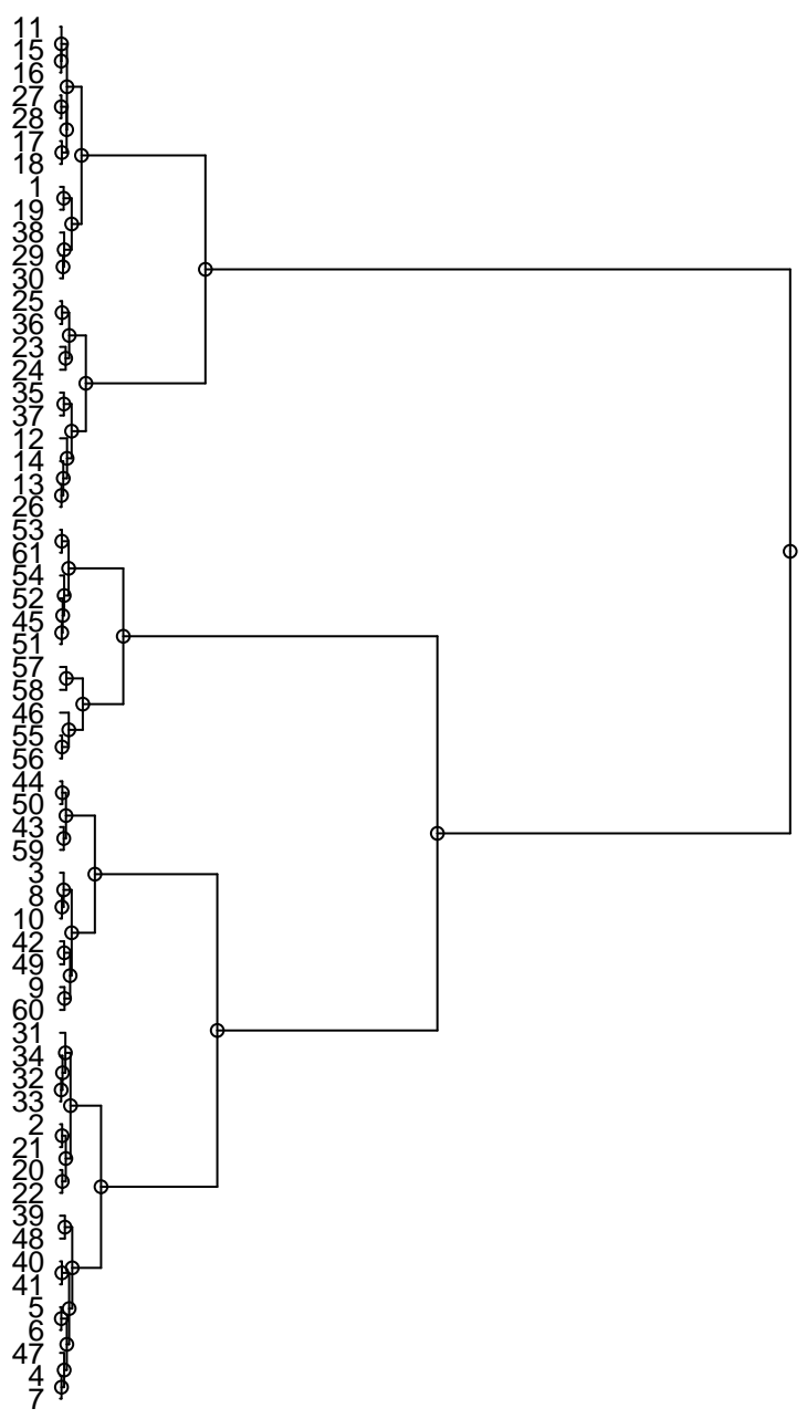
Dendrogram
