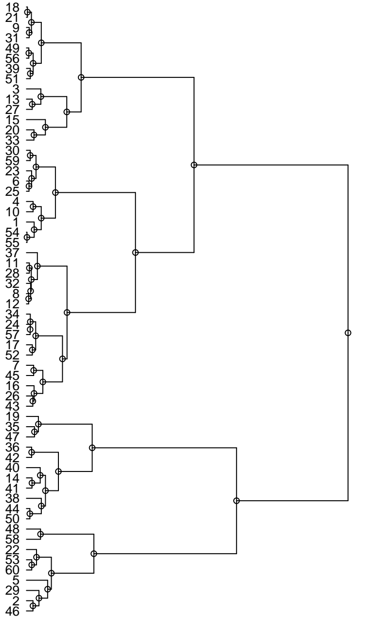
Dendrogram
