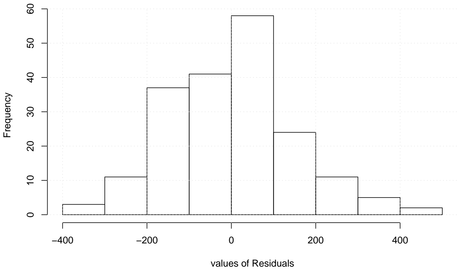
Residual Histogram
