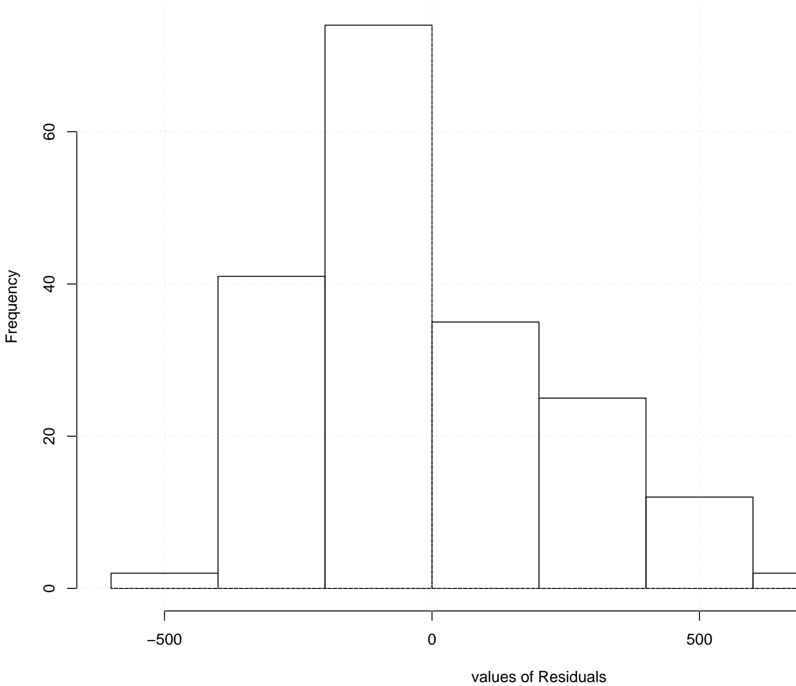
Residual Histogram
