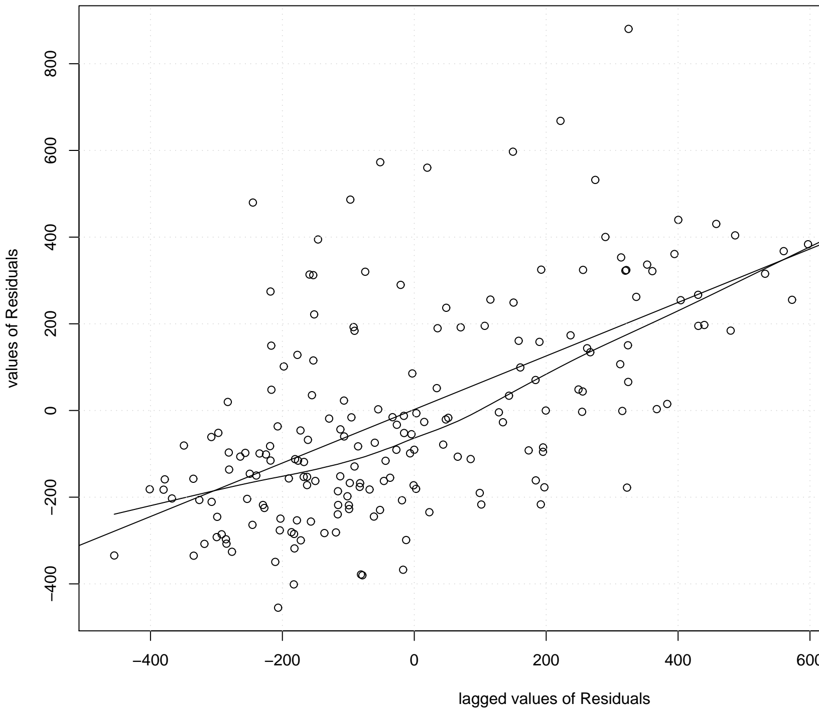
Residual Lag plot, lowess, and regression line
