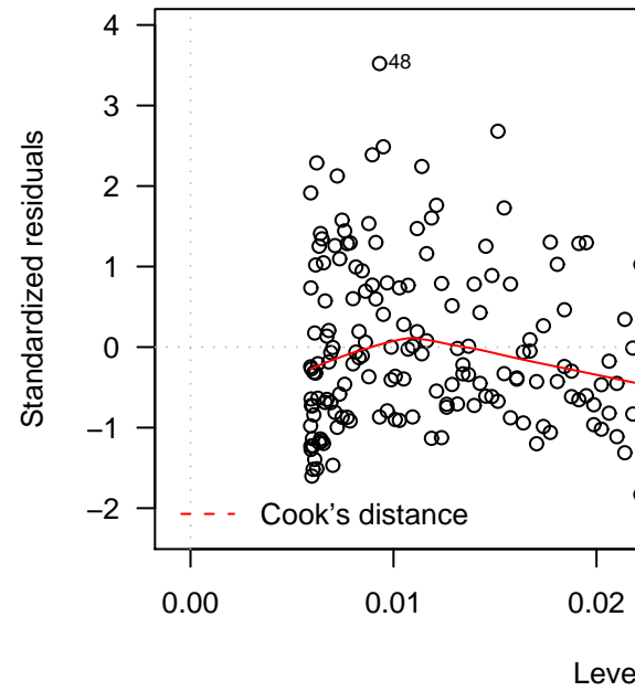
Residuals v
