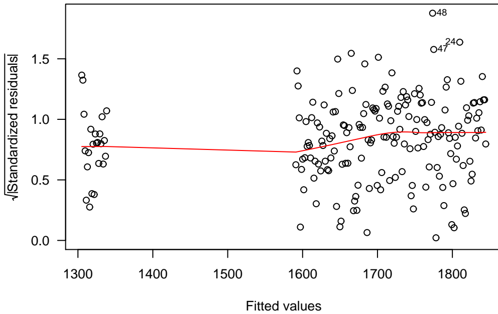
Scale-Location
