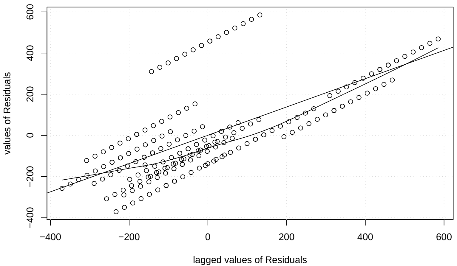
Residual Lag plot, lowess, and regression line
