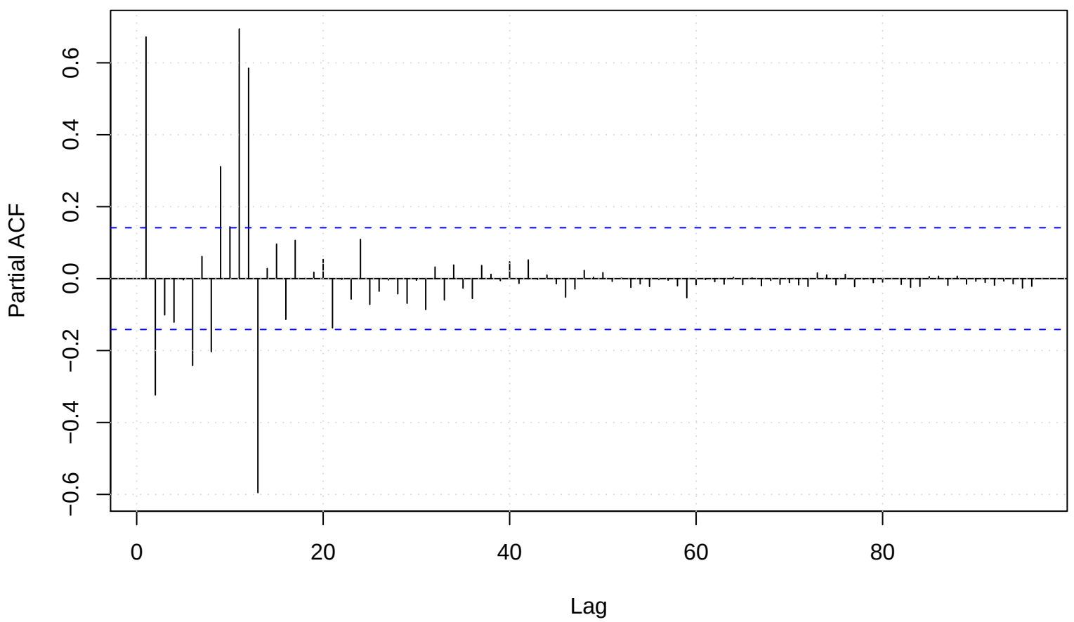
Residual Partial Autocorrelation Function
