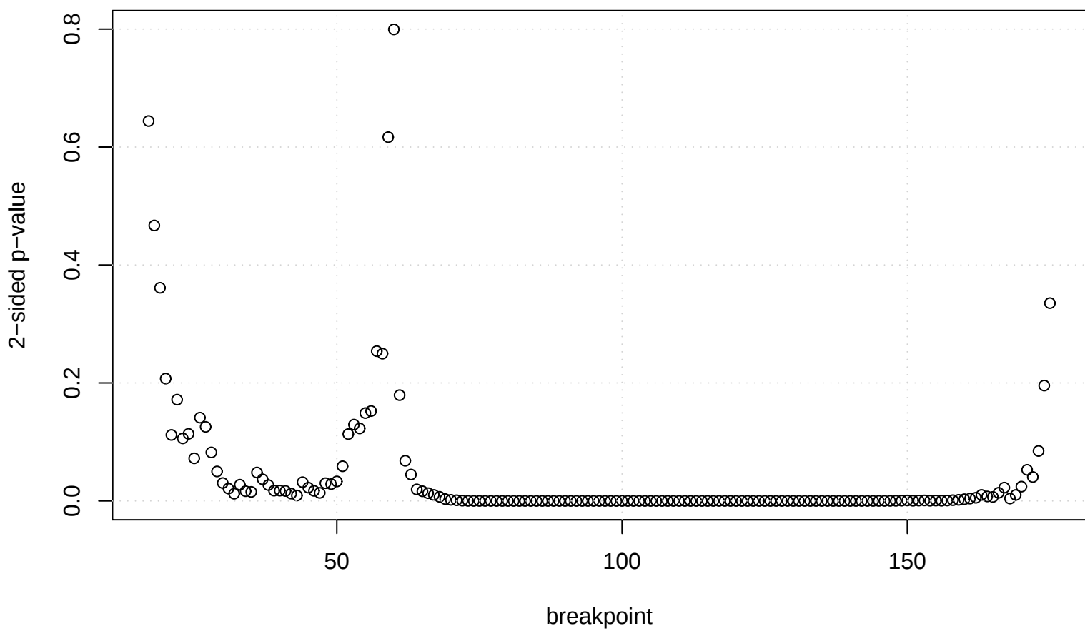
Goldfeld-Quandt test
