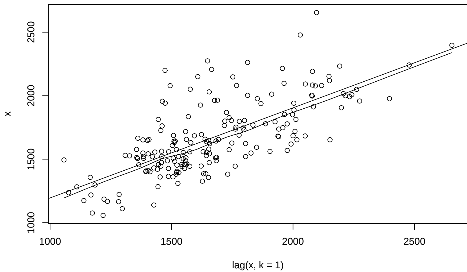
Lag plot (k=1), lowess, and regression line
