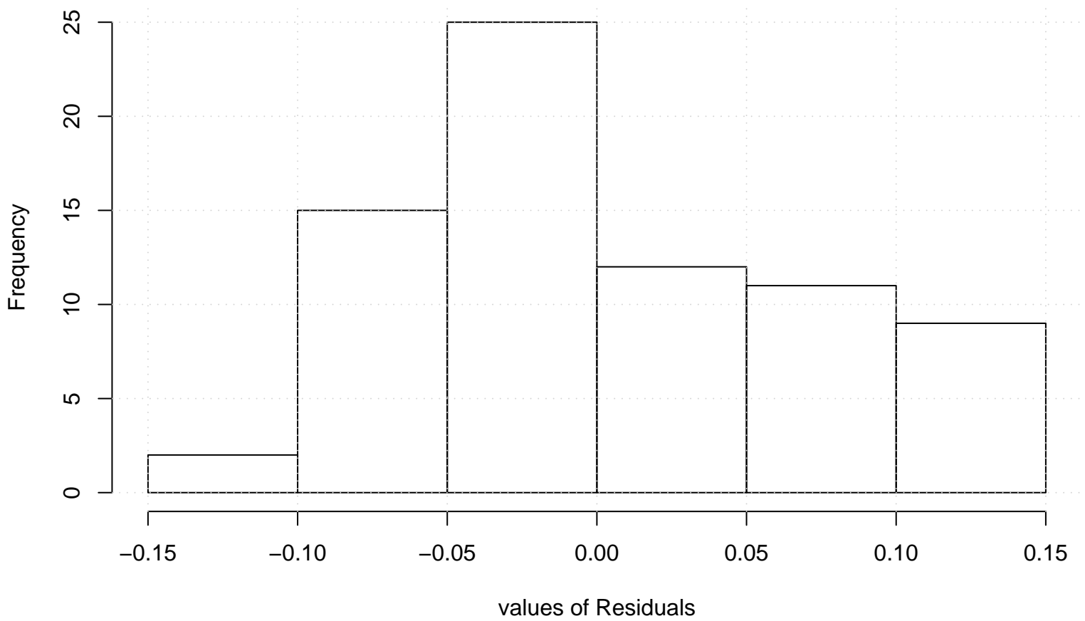
Residual Histogram
