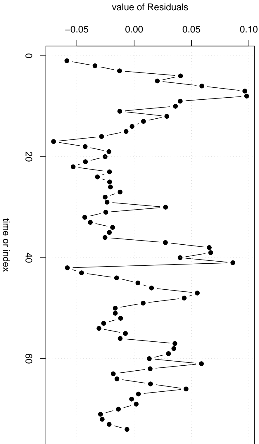
Residuals
