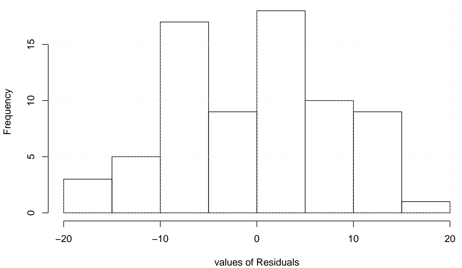
Residual Histogram
